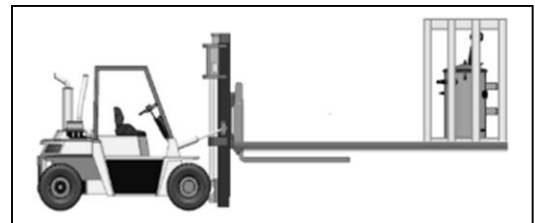
Figure 21: Proper way to pull a transformer in the download
