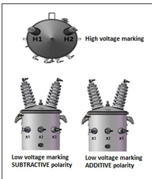
Figure 41: ANSI marking
