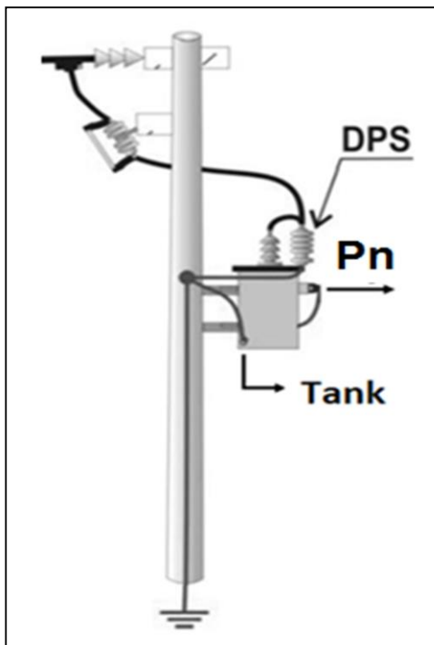
Figure 49: Grounding system
