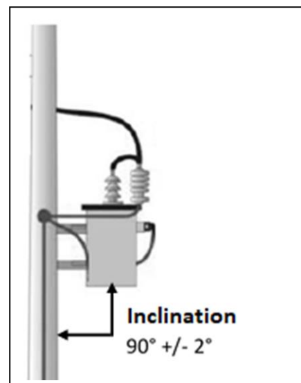
Figure 48: Inclination Degree
